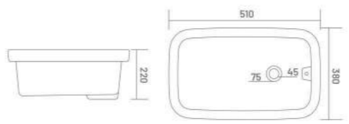
LAB SINK 20" x 15" x 8"
