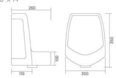
CORNER URINAL Urinal 12" x 10" x 14"
