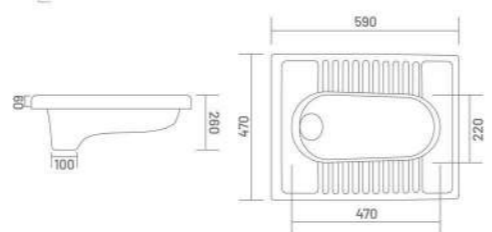
ORISSA PAN - 23" Pan 23" x 19" x 10"
