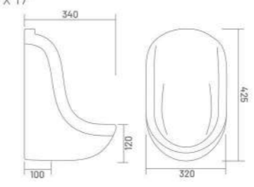
NANO LARGE Urinal 13" x 13" x 17"
