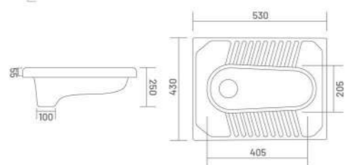
ORISSA PAN - 20" Pan 20" x 17" x 10"
