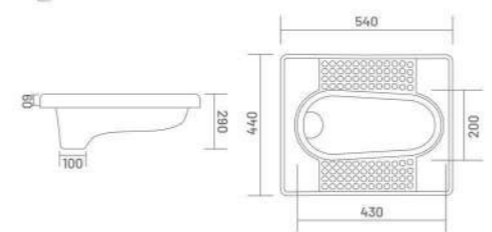
AQUA PAN - 21" Pan 21" x 18" x 12"
