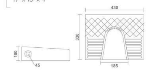
SQUATTING Urinal 17" x 13" x 4"
